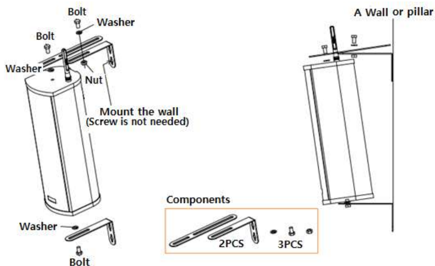
Figure 5-1) mount MDS-2400/1400 to a wall
